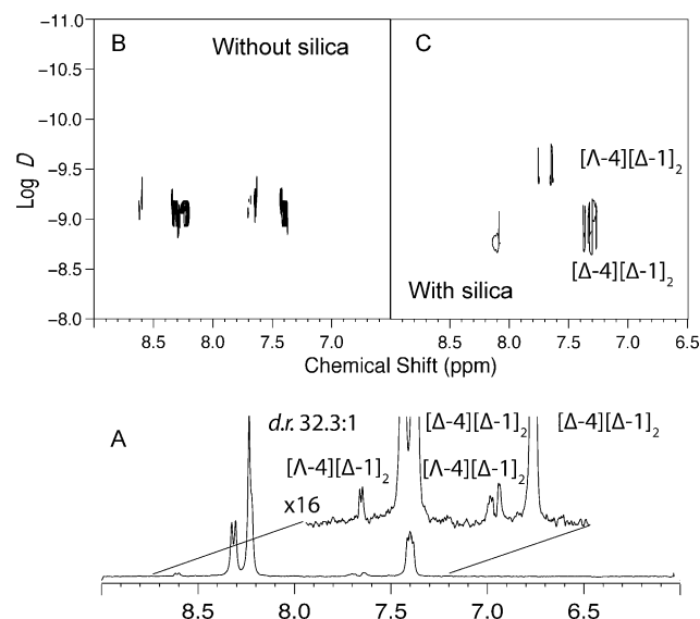
Figure 4. Spectra (9.0–6.5 ppm, \text{CD}_2\text{Cl}_2 ) of equilibrating iron diastereomeric pairs [\Delta-4][\Delta-1]_2 and [\Lambda-4][\Delta-1]_2 . A) ^1\text{H} NMR spectrum (d.r. 32.3:1). B) Solution-state DOSY spectra with a diffusion time of 100 ms and a PFG duration of about 1.2 ms. C) Chromatographic NMR spectroscopy (bare silica, f=2.0 ) with a diffusion time of 180 ms and a PFG duration of 2 ms.
